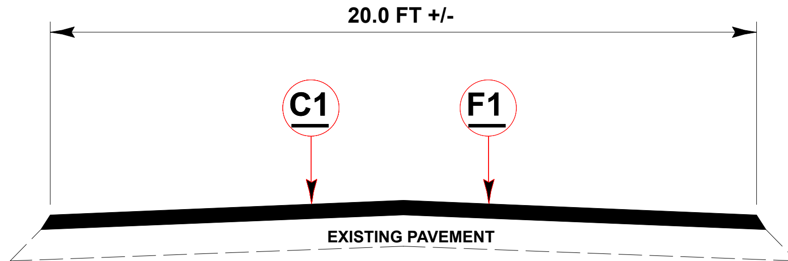
TYPICAL SECTION # 2 MAP(S) # 5 - 7
